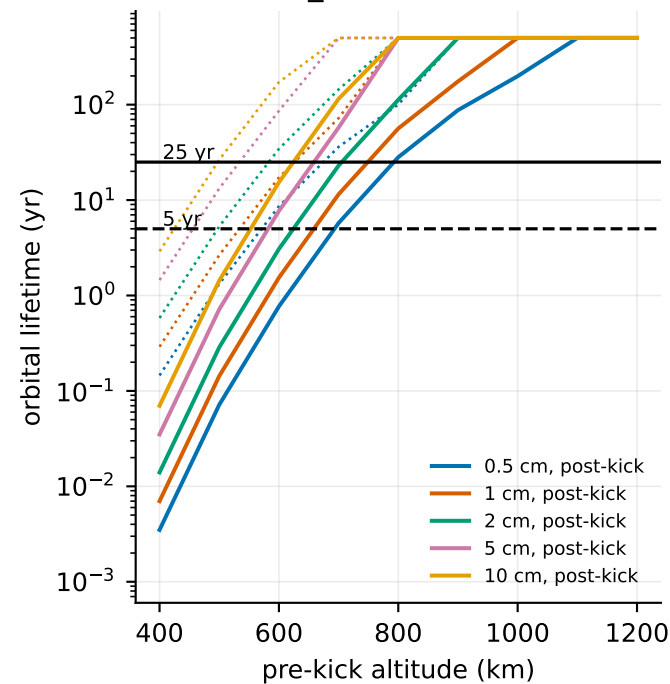
SIM-2: lifetime after a 200 km kick (solid) vs. undisturbed (dotted); values at 500 yr are capped solar_min (F10.7=70) nominal (F10.7=150) solar_max (F10.7=250)
