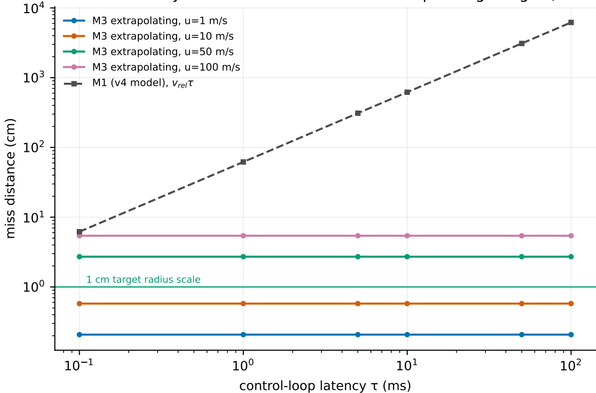
SIM-4: the v4 latency cliff versus the co-orbital extrapolating budget ( R = 10 m)
