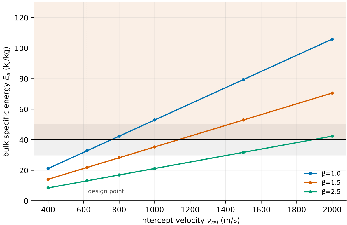
SIM-5: distance to the catastrophic threshold at 800 km (grey band = 30-50 kJ/kg threshold uncertainty)
