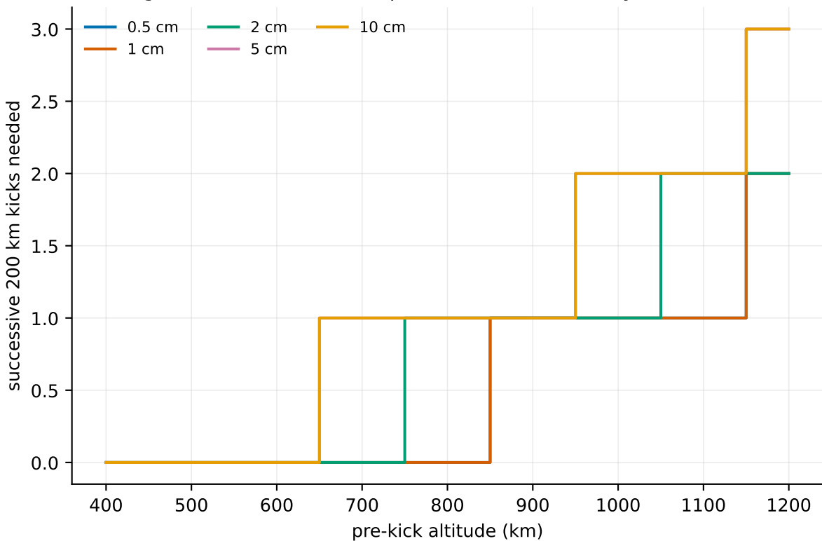
SIM-2: staged deorbit — kicks required to meet the 25-yr rule (nominal solar)
