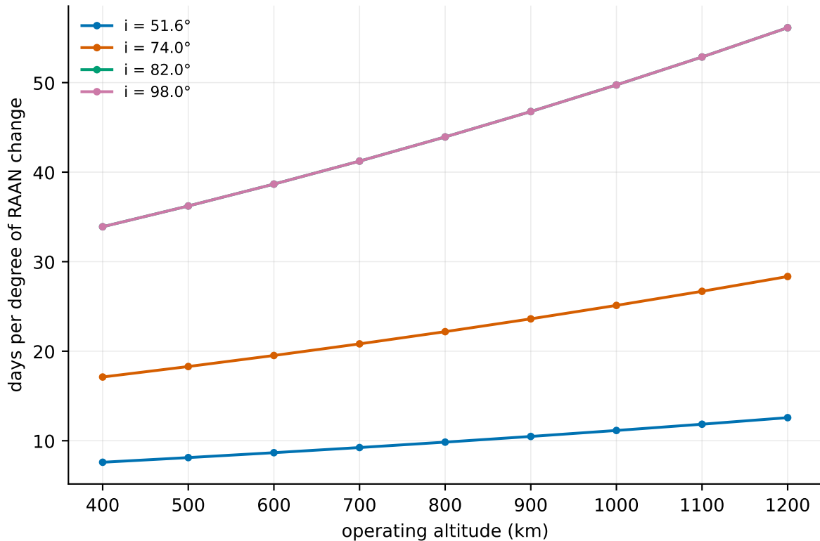
SIM-11: RAAN access via differential J2 drift (50 km parking offset, ~50 m/s round trip)
