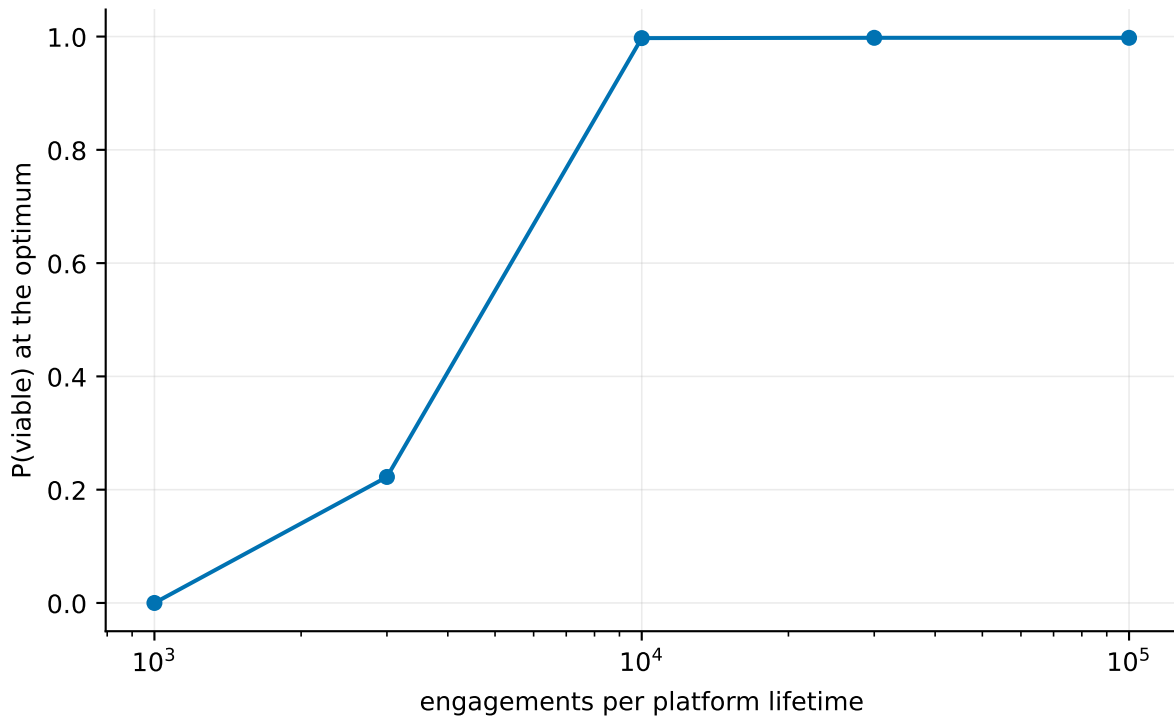
SIM-13: the dominant term is programmatic, not physical
