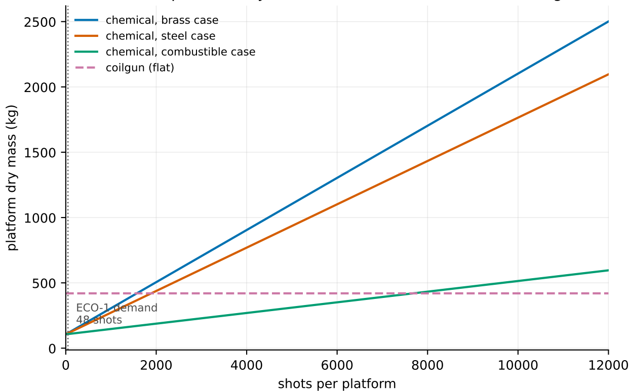
LNCH-02: platform dry mass vs shot count, chemical vs coilgun
