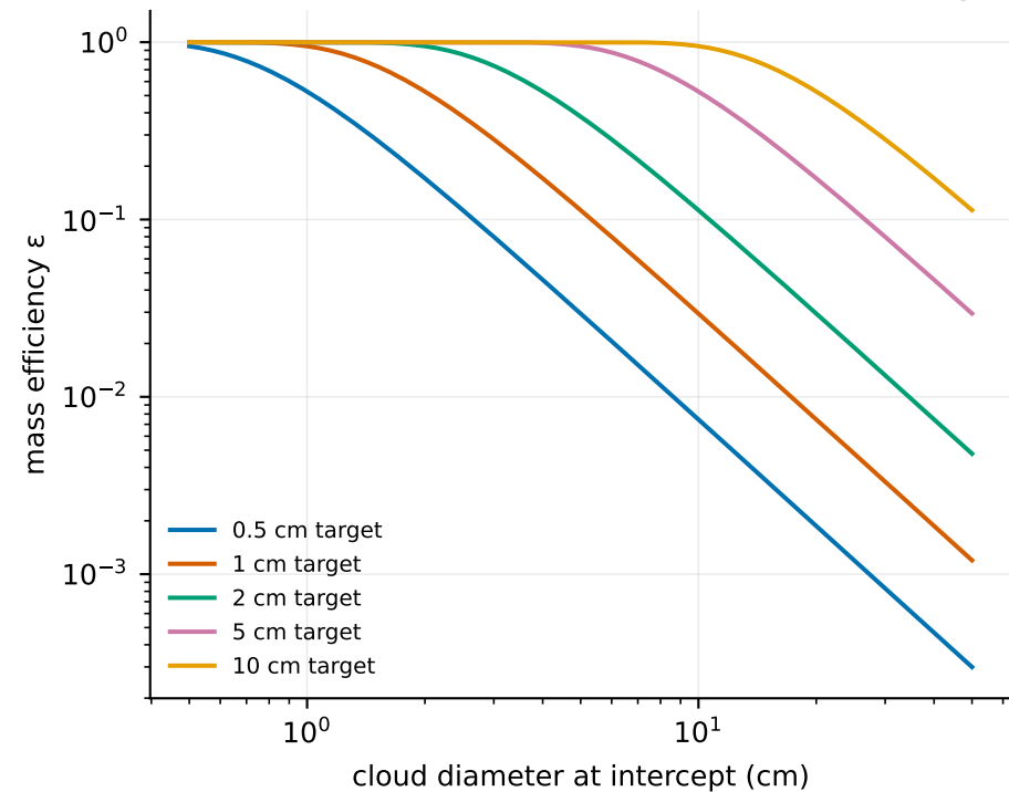
Fraction of launched mass that lands on the target
