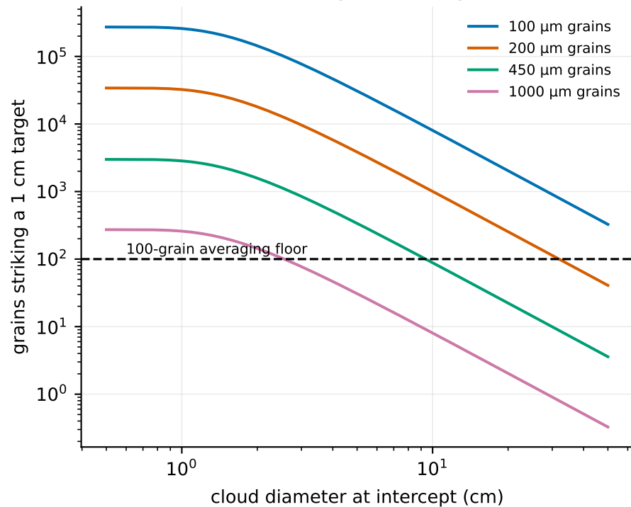
Grains on target for a 3 g shot
