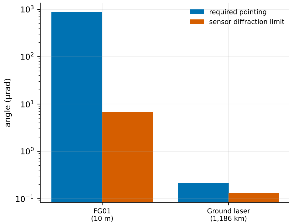
Headroom against the physics of the optics
