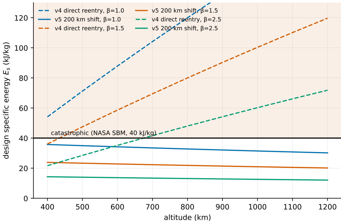
SIM-0: the v4→v5 pivot, at the common design point v_{rel}=619 m/s, \gamma=2
