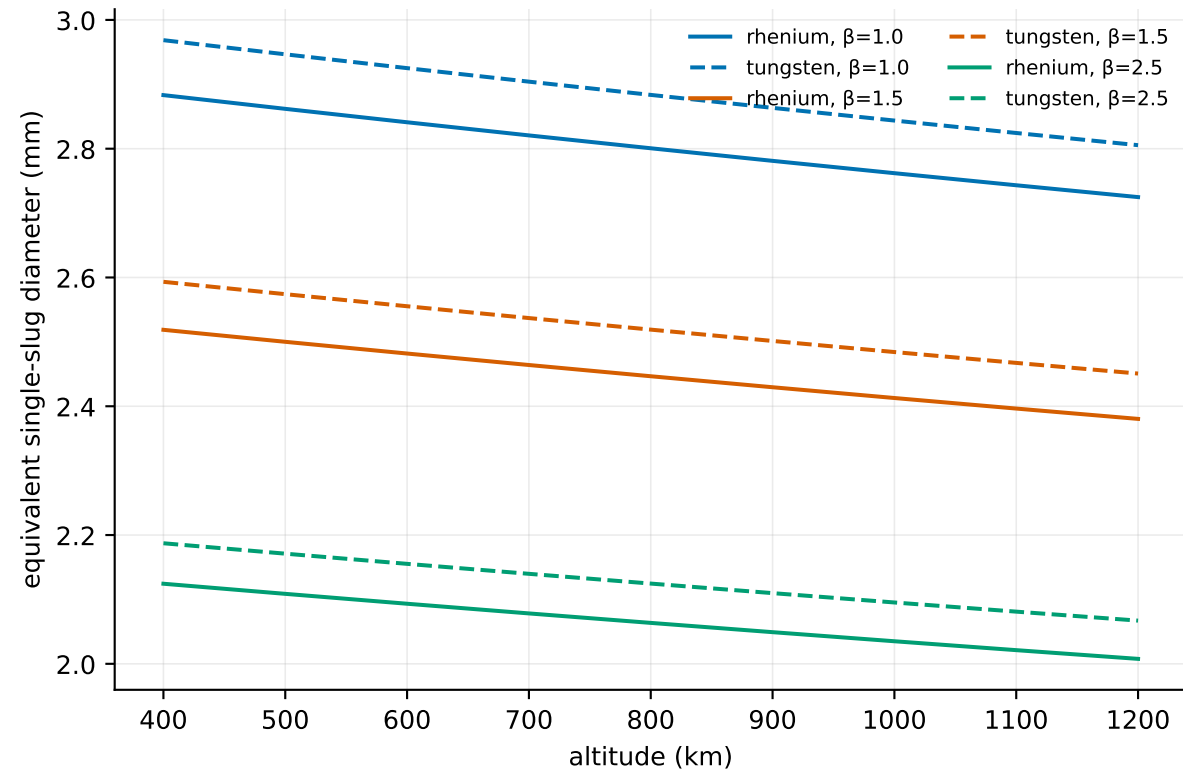
SIM-1: equivalent compact-projectile size, 1 cm Al target, v_{rel}=619 m/s
