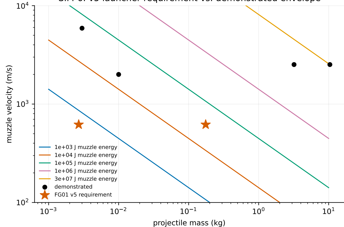
SIM-6: v5 launcher requirement vs. demonstrated envelope
