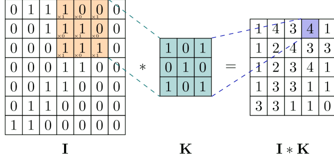
Figure 7 – Illustration of the convolution operation in a convolutional neural network. (RIEBESSELL, 2022)
