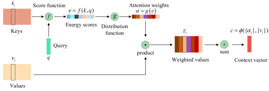
Figure 11 – Diagram of the attention mechanism showing query, key, value vectors, and the computation of the context vector. (NIU; ZHONG; YU, 2021)
