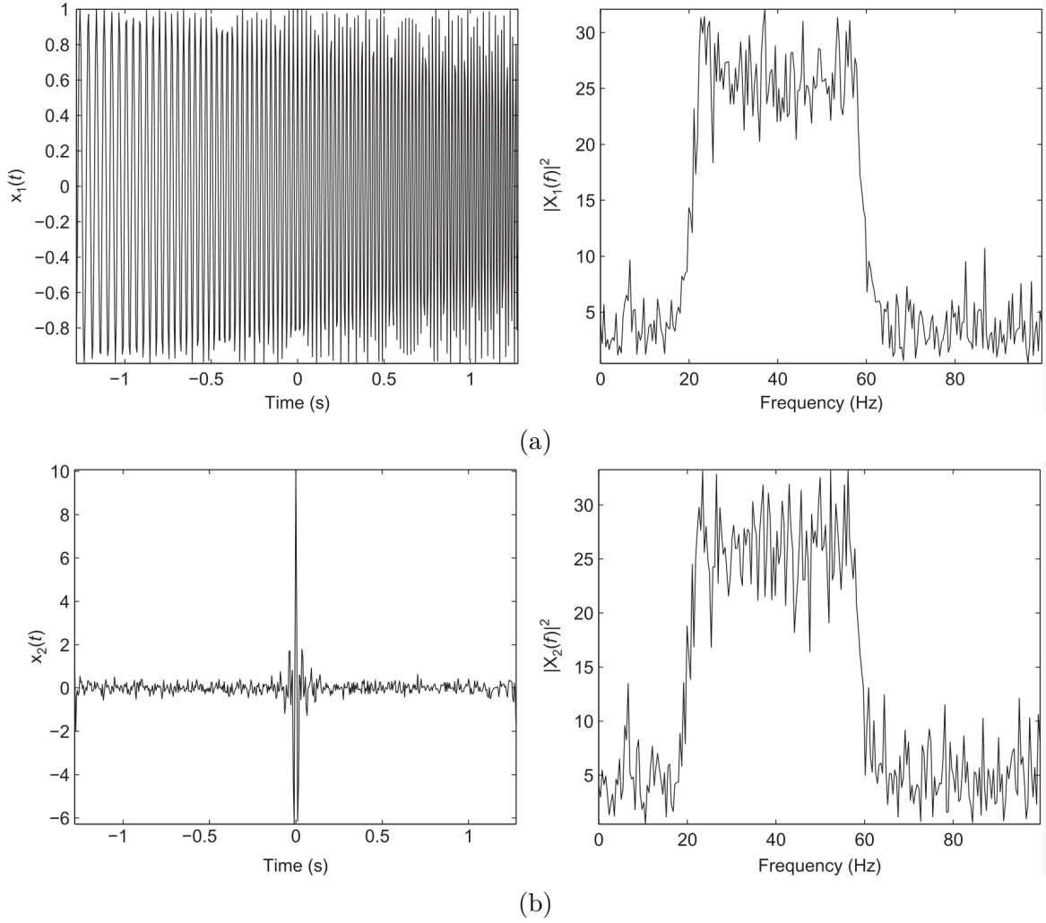
Figure 5 – Time and frequency representations of the signals defined in Equations 2.6 and 2.7. (a) Time and frequency representations of the signal x_1 . (b) Time and frequency representations of the signal x_2 .
