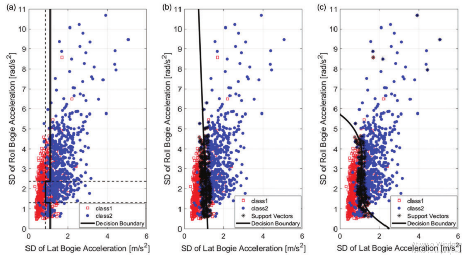
Figure 24 – Classification results of the three classifiers on the test set. (a) the decision boundary for the decision tree. (b) the decision boundary for the linear SVM. (c) the decision boundary for the Gaussian SVM. (ROSA et al., 2021)
