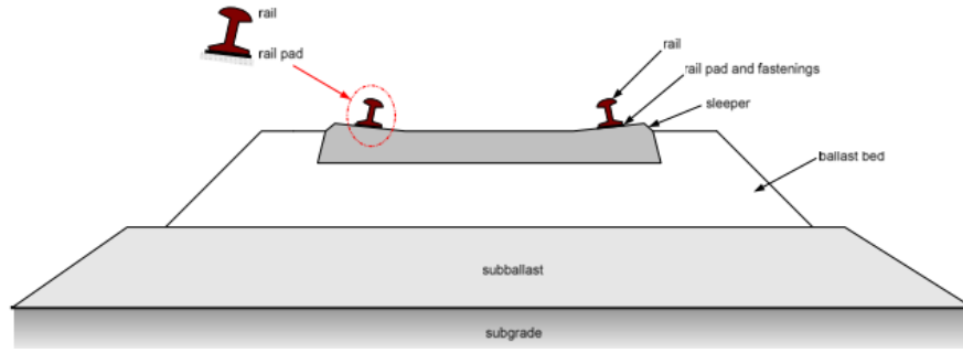
Figure 12 – Main railway track components, including superstructure and substructure. (KAEWUNRUEN 1 ; REMENNIKOV 1 , 2008)
