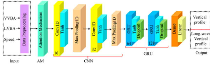
Figure 21 – Model architecture utilized to reconstruct the track irregularity (HAO et al., 2023).
