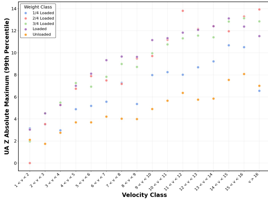
Figure 16 – Effect of wagon mass on the relationship between acceleration and velocity for freight trains. The data points represent the 99th percentile of the absolute maximum vertical acceleration for each velocity class, colored by wagon mass class.
