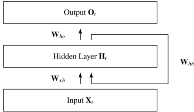
Figure 8 – Architecture of a recurrent neural network showing the recurrent connections between hidden states. Adapted from (SCHMIDT, 2019)
