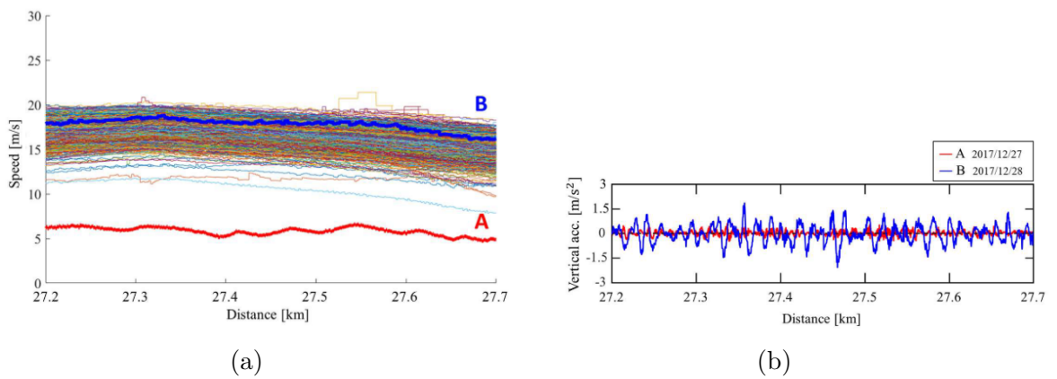
Figure 13 – Example of how velocity differences affect acceleration measurements on the same track segment. (a) shows the two velocity profiles, A and B. (b) illustrates the corresponding acceleration measurements for each profile. Adapted from (ONO et al., 2023).
