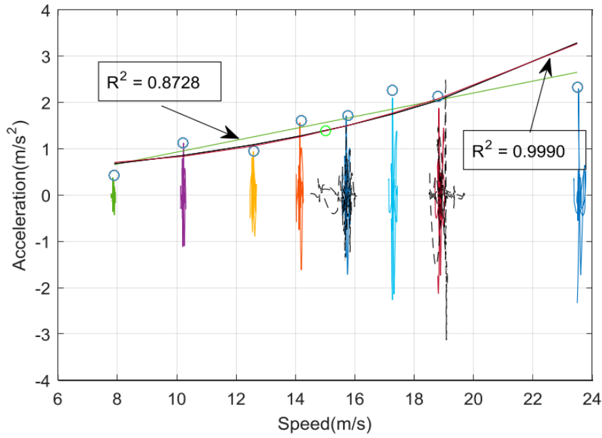
Figure 15 – Effect of train velocity on measured acceleration compared with simulation results and the linear and exponential model fitted to the maximum acceleration values with their corresponding R^2 values (BALOUCHI; BEVAN; FORMSTON, 2021).
