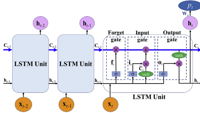
Figure 9 – Structure of an LSTM cell with input, forget, and output gates. Adapted from (WEI et al., 2021)
