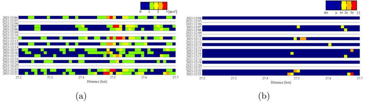
Figure 14 – Reduction of false positives in anomaly detection after velocity correction. (a) shows the heatmap of the acceleration measurements before correction, while (b) shows the heatmap after correction. Adapted from (ONO et al., 2023).
