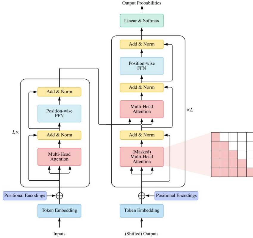
Figure 11 – Architecture of the vanilla Transformer model, with encoder and decoder components. (LIN et al., 2021)
