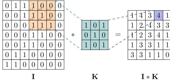
Figure 6 – Illustration of the convolution operation in a convolutional neural network. (RIEBESSELL, 2022)
