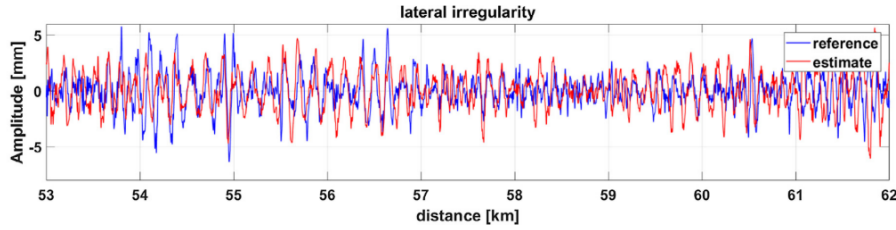
Figure 17 – Reconstruction of lateral irregularities using the Frequency Response Function method (De Rosa; ALFI; BRUNI, 2019).
