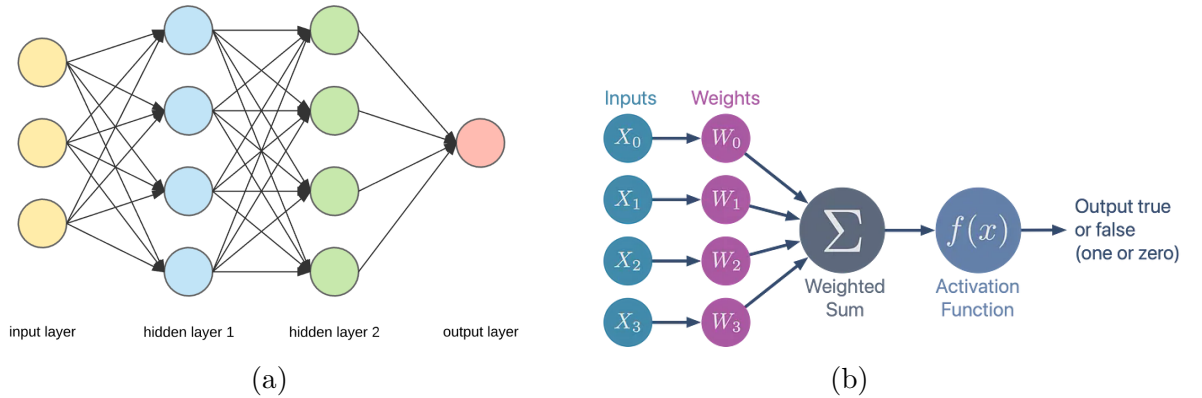
Figure 5 – Structure of a neural network. (a) Fully connected perceptrons arranged in layers (P., 2025). (b) Perceptron with activation function (WEAVER, 2024).
