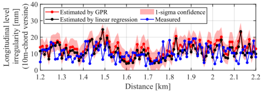
Figure 20 – Regression results comparing predicted and actual track irregularities from real measurement data. (TSUNASHIMA; YAGURA, 2024)
