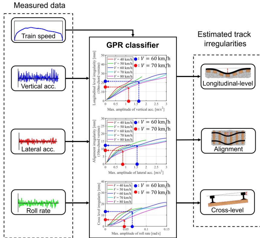
Figure 19 – Track irregularity prediction using Gaussian Process Regression for different vehicle speeds (TSUNASHIMA; YAGURA, 2024).
