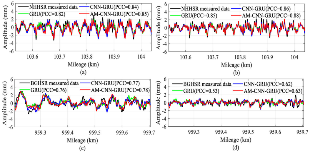
Figure 22 – Reconstruction results comparing the proposed model (red) with two simpler models (blue and green) and the original measurement (black). (a) and (b) show vertical and lateral, respectively, irregularities reconstruction for the NHHSR line. (c) and (d) show the vertical and lateral, respectively, irregularities reconstruction for the BGHSR line (HAO et al., 2023).
