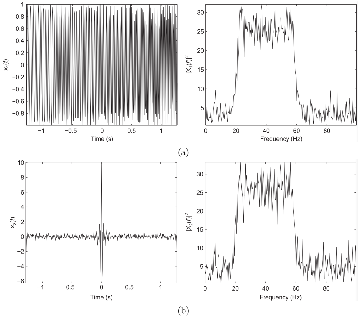
Figure 5 – Time and frequency representations of the signals defined in Equations 2.9 and 2.10. (a) Time and frequency representations of the signal x_1 . (b) Time and frequency representations of the signal x_2 .
