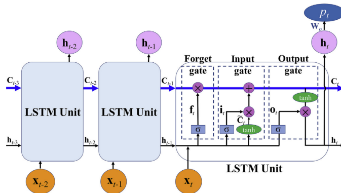
Figure 8 – Structure of an LSTM cell with input, forget, and output gates. Adapted from (WEI et al., 2021)
