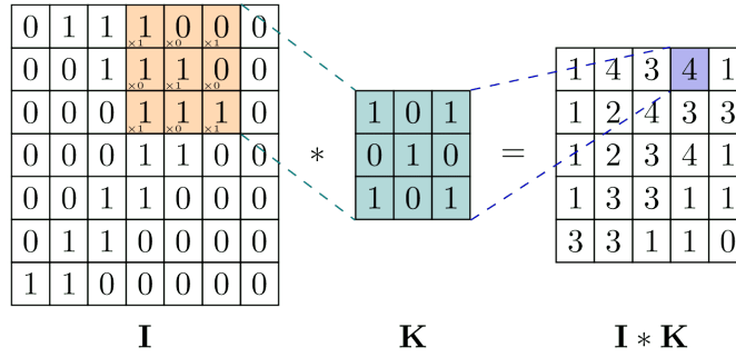
Figure 5 – Illustration of the convolution operation in a convolutional neural network. (RIEBESSELL, 2022)
