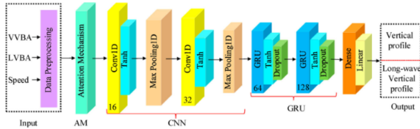
Figure 20 – Model architecture utilized to reconstruct the track irregularity (HAO et al., 2023).
