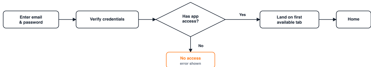
Fig. 2 — Login always resolves to whichever tab the role actually grants, e.g. Attendance for a role without Home access — never a hardcoded screen a role can't use.
