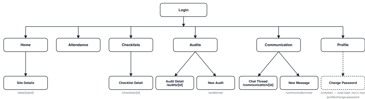
Fig. 1 — Full screen hierarchy. Dashed = built but currently unreachable from navigation.
