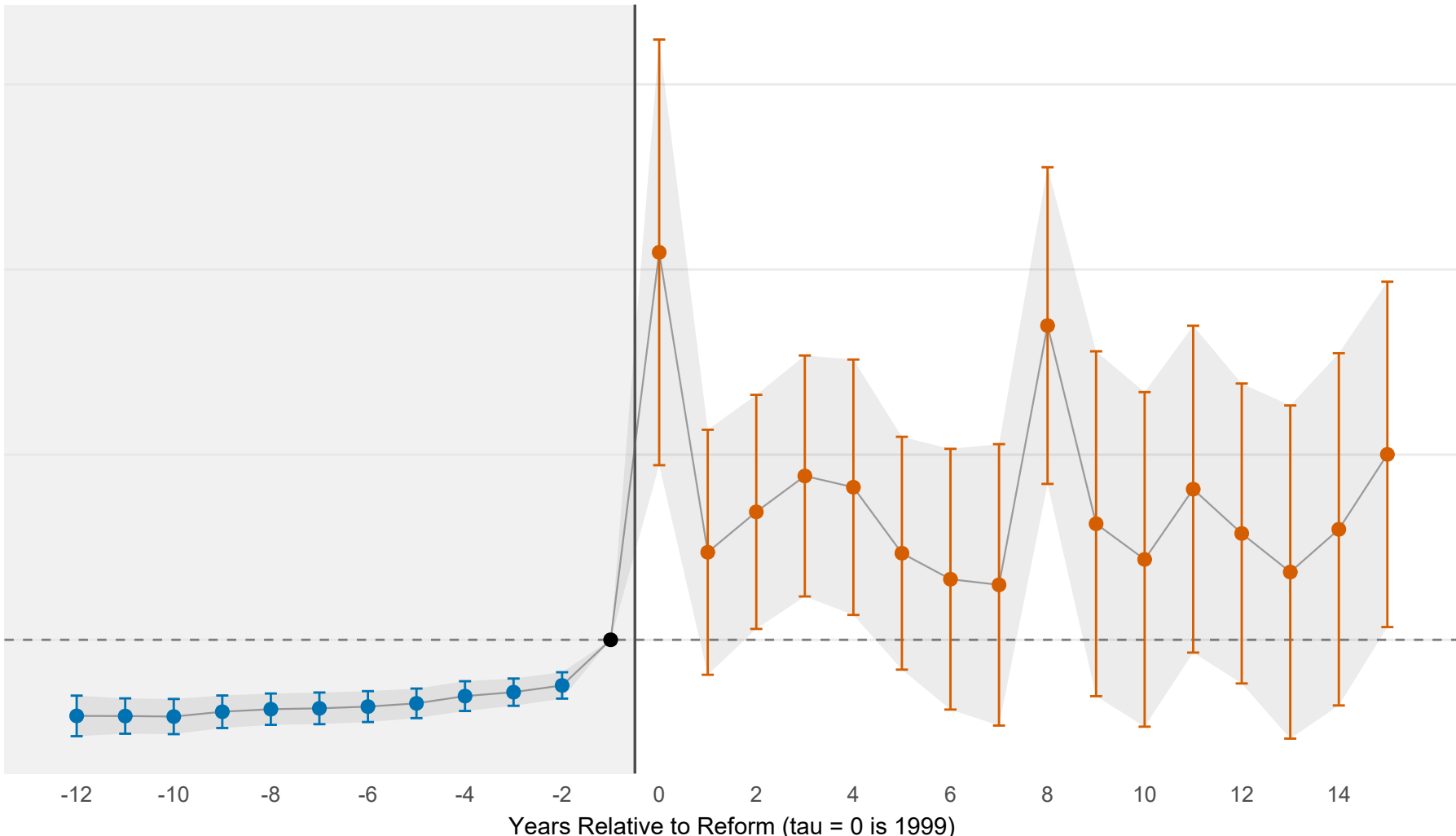
Effect on Facility Exit Probability (Closes Entirely)
