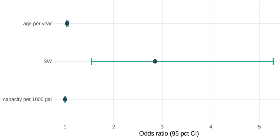
Figure 3: Removal odds ratios, within facility
