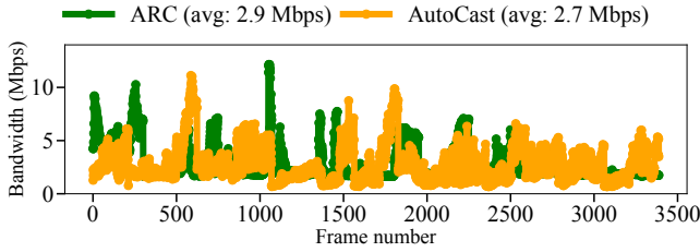
Figure 21: ARC and AutoCast comparison: bandwidth consumption per vehicle for synthetic traces.
