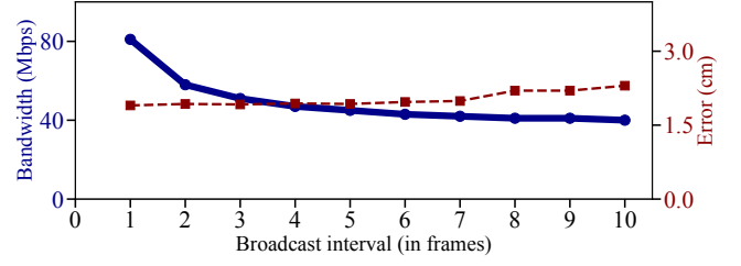
Figure 22: Impact of anchor broadcast frequency on ARC’s alignment error and bandwidth requirements.
