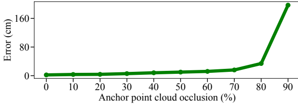
Figure 23: Impact of anchor occlusion on ARC's alignment accuracy.
