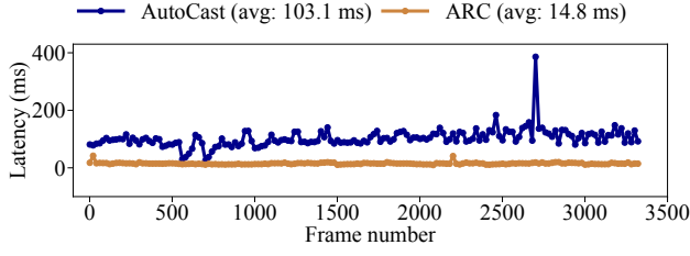
Figure 19: Compute latency of ARC and AutoCast on the CARLA traces.
