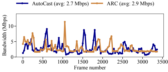
Figure 21: ARC and AutoCast comparison: bandwidth consumption per vehicle for synthetic traces.
