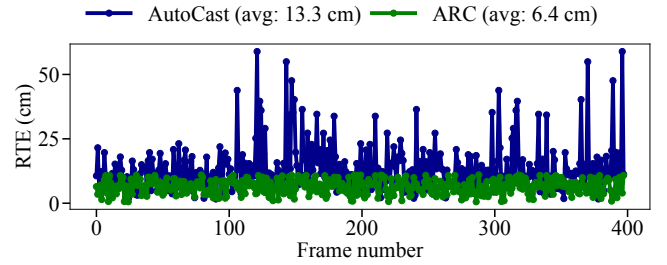
Figure 17: Comparison of ARC and AutoCast RTE on the real-world traces.
