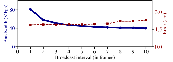
Figure 22: Impact of anchor broadcast frequency on ARC’s alignment error and bandwidth requirements.
