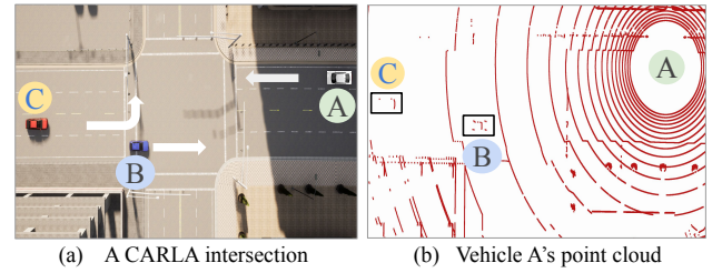
Figure 27: A CARLA scenario, where vehicles A, B, and C are approaching an intersection. In vehicle A's point cloud, both vehicle B and C are visible.
