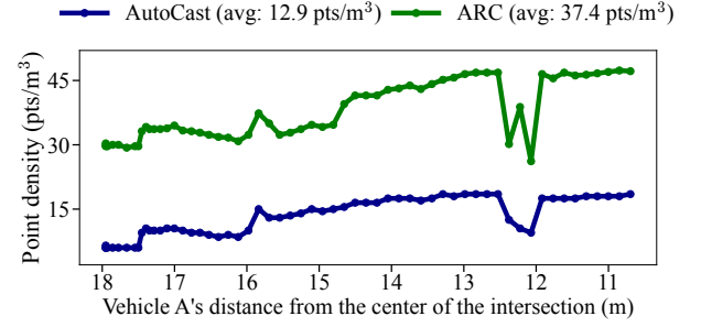
Figure 26: Comparison of AutoCast and ARC showing the mean point density of objects visible to A in each frame in the scenario shown in Fig. 27.
