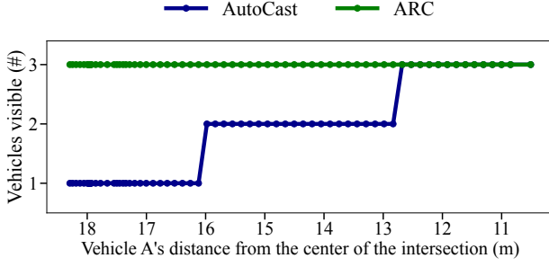
Figure 25: Comparison of AutoCast and ARC in the scenario shown in Fig. 24, with the number of vehicles visible to vehicle A in each frame.
