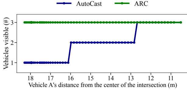
Figure 25: Comparison of AutoCast and ARC in the scenario shown in Fig. 24. It shows the number of vehicles visible to vehicle A in each frame as a function of its distance from the intersection center.
