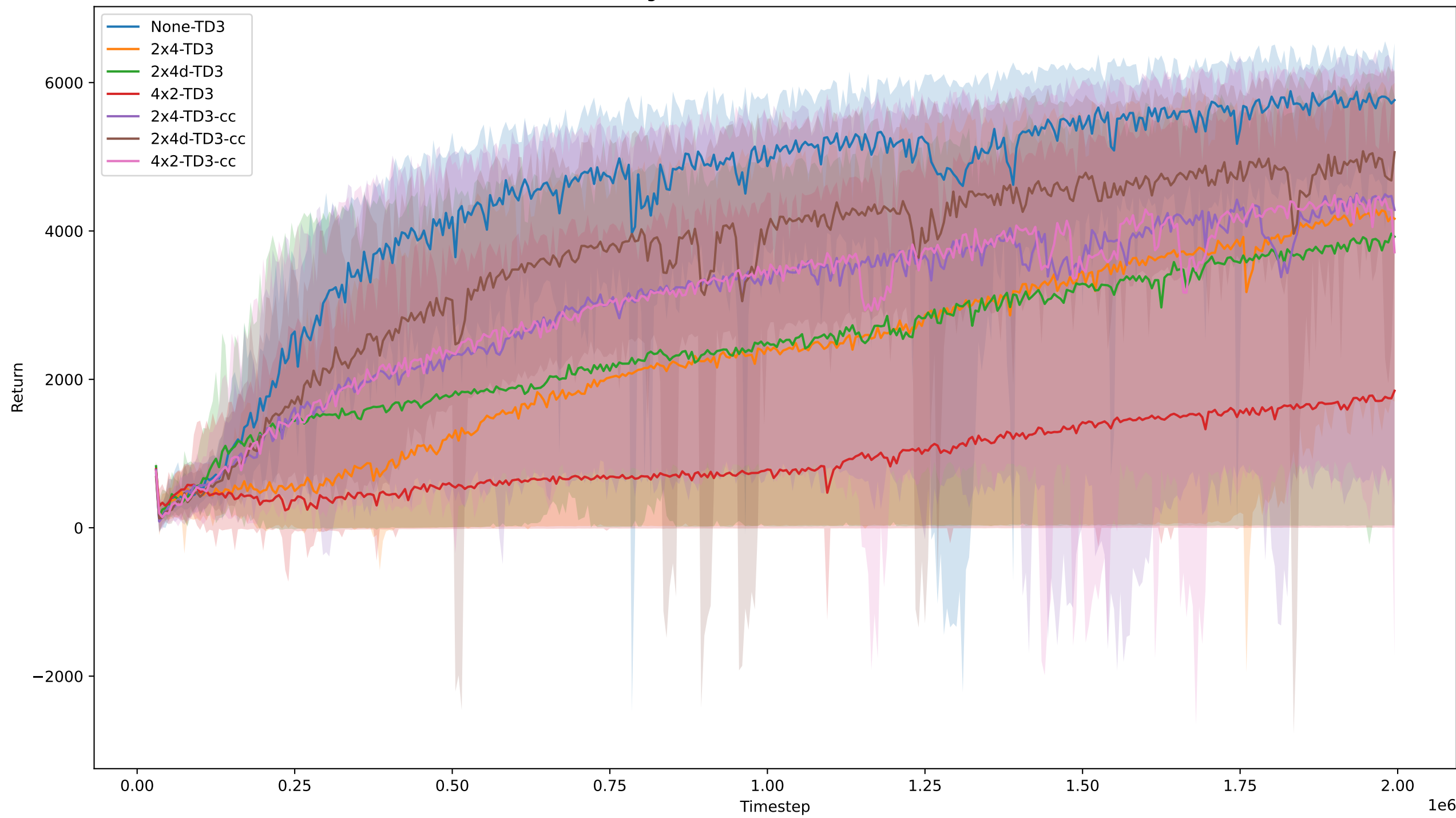
average over 10 statistical runs, on Ant
