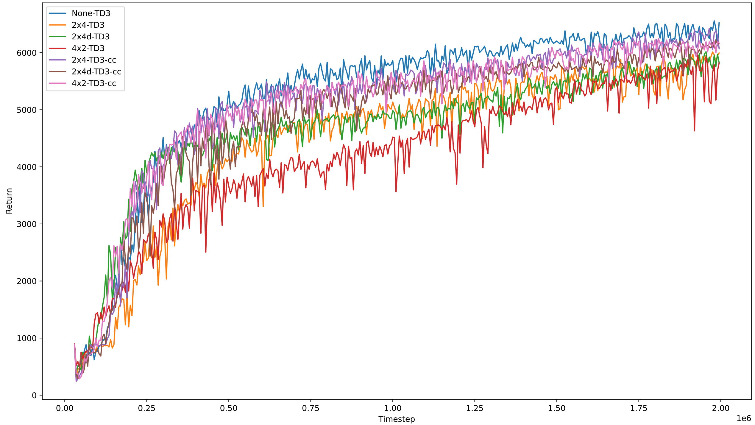
max over 10 statistical runs, on Ant
