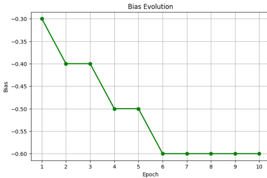
Figure 6: Bias Evolution
