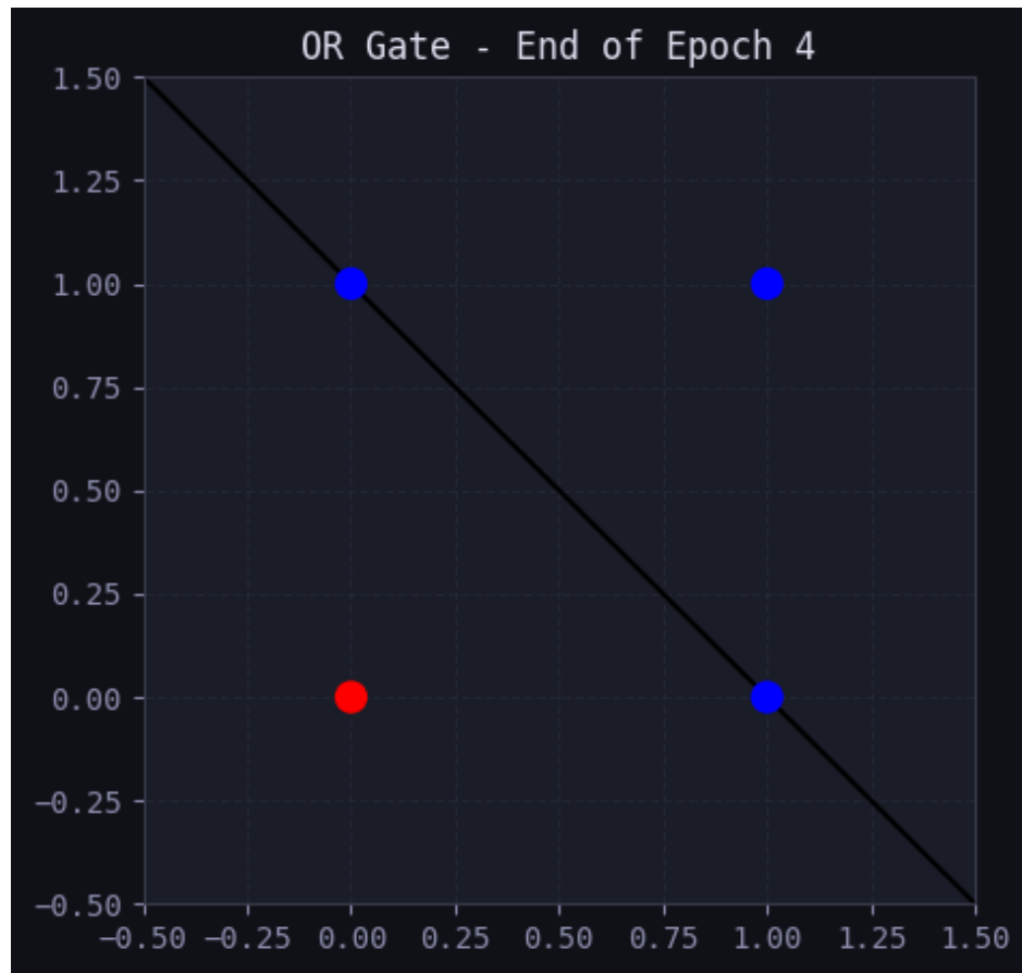
Figure 10: OR Gate Decision Boundary Progression
