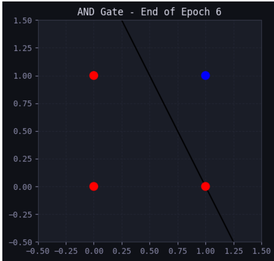
Figure 11: AND Gate Decision Boundary Progression
