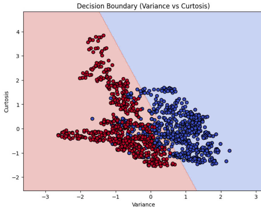
Figure 9: Decision Boundary
