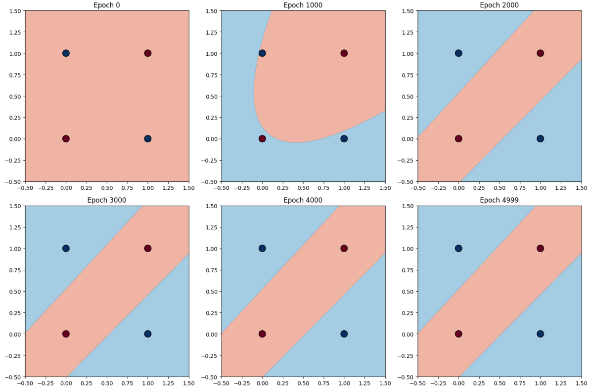
Figure 11: XOR gate implementation using MLP
