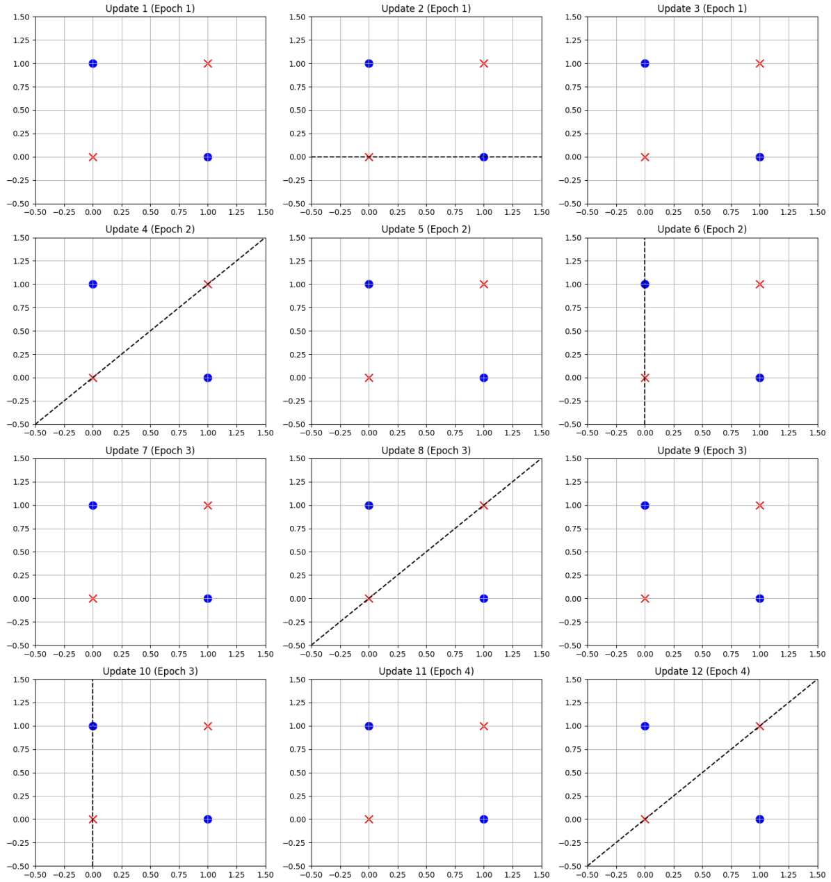
Figure 10: XOR gate implementation using SLP - Failed Convergence
