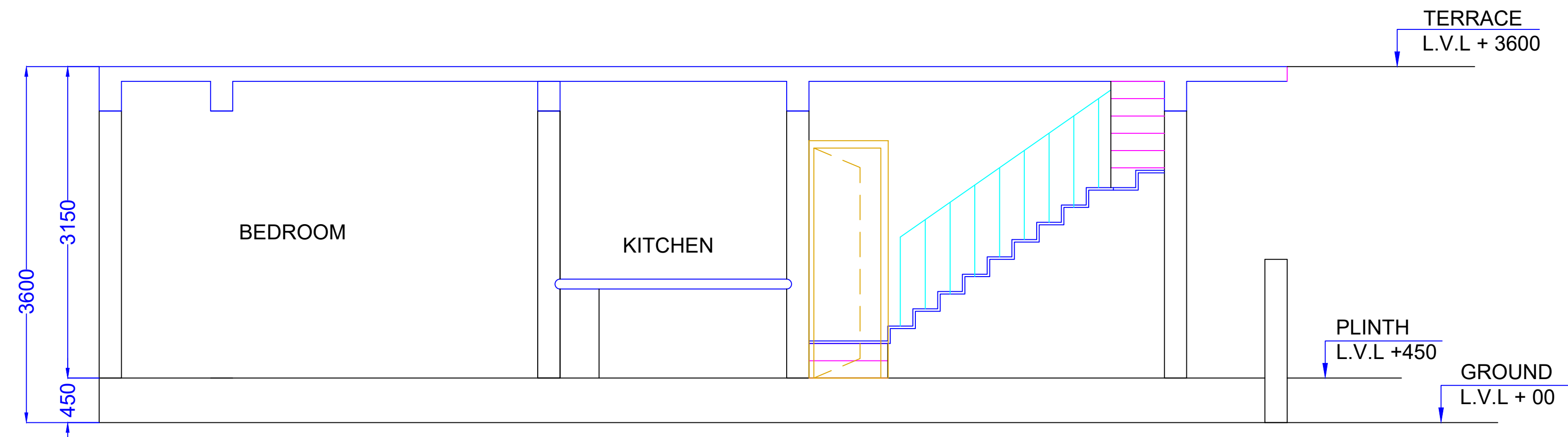
SECTION AT X-X'
