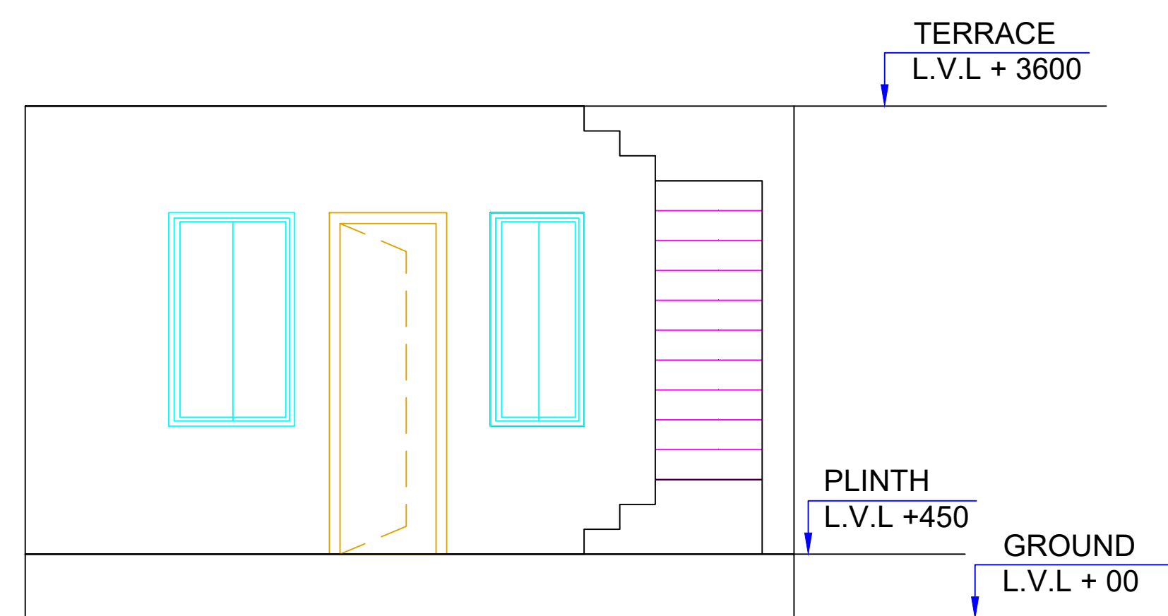
FRONT ELEVATION
