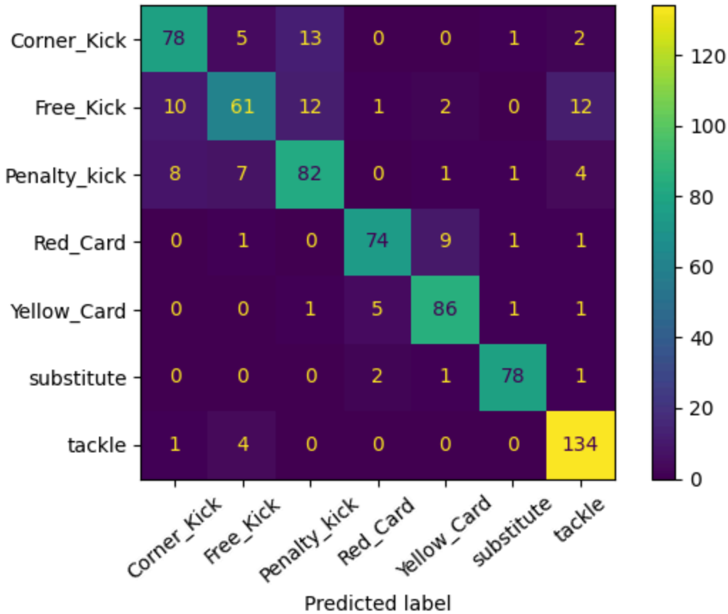
convnext Confusion Matrix
