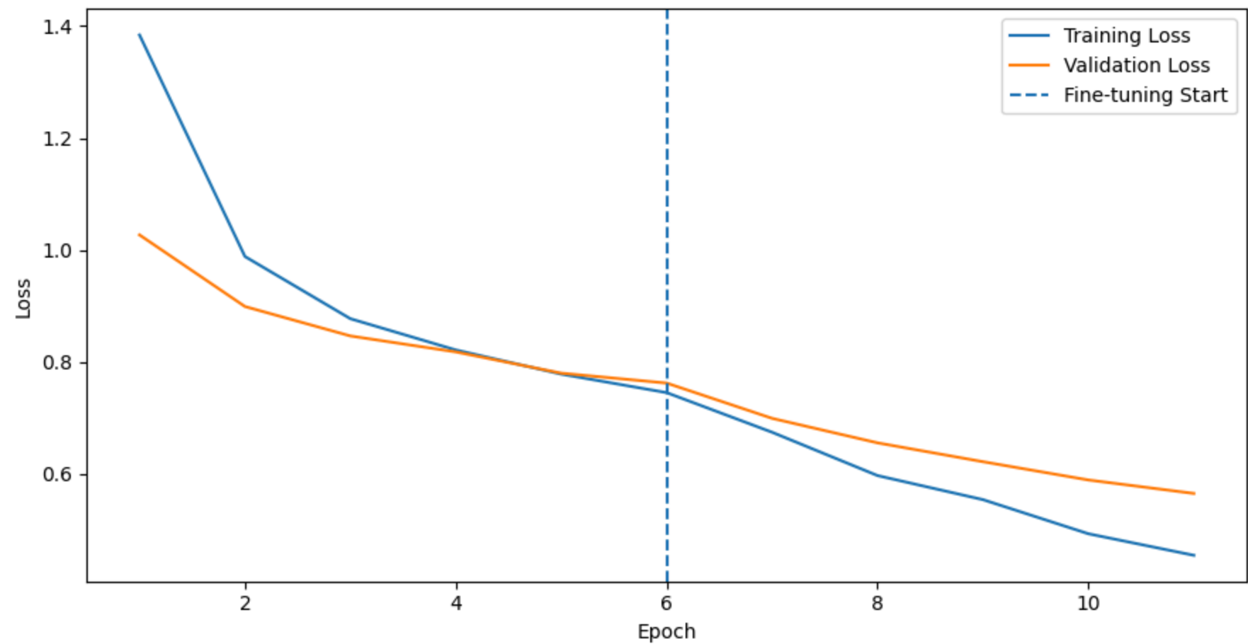
convnext Loss
