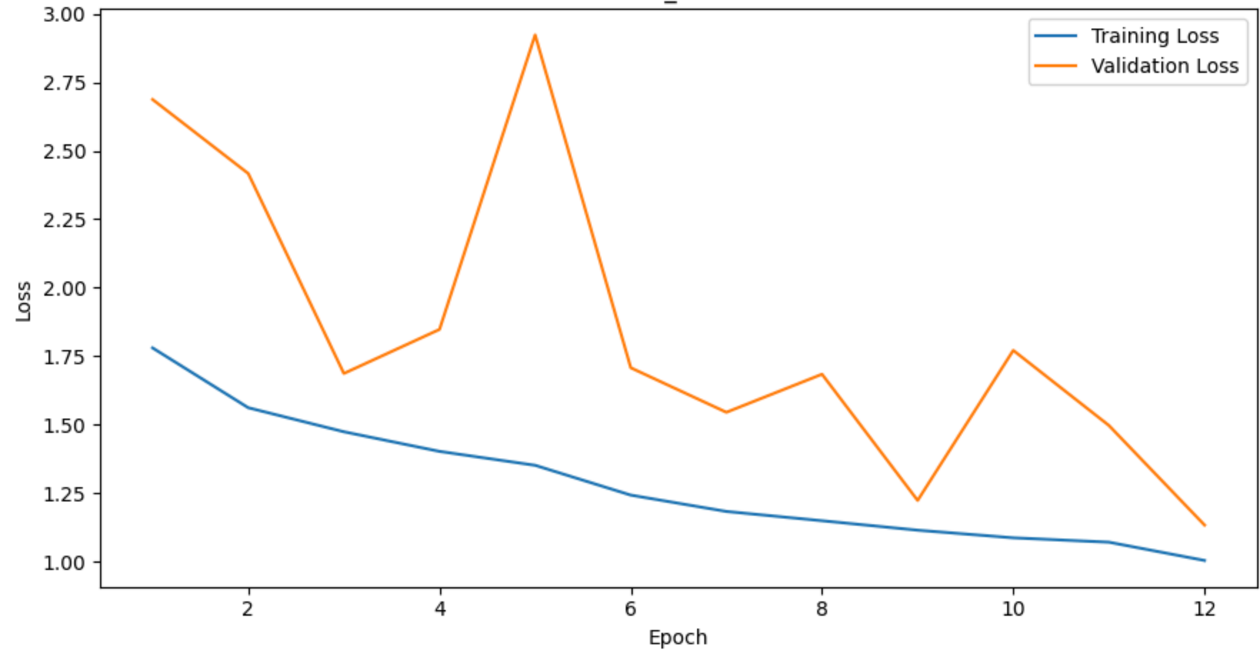
custom_cnn Loss
