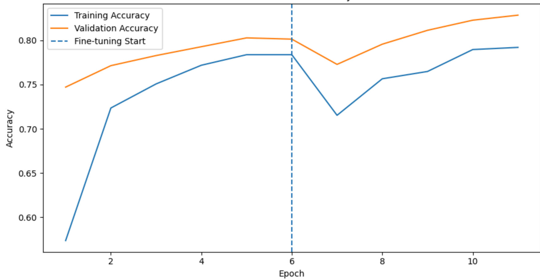
efficientnetv2 Accuracy
