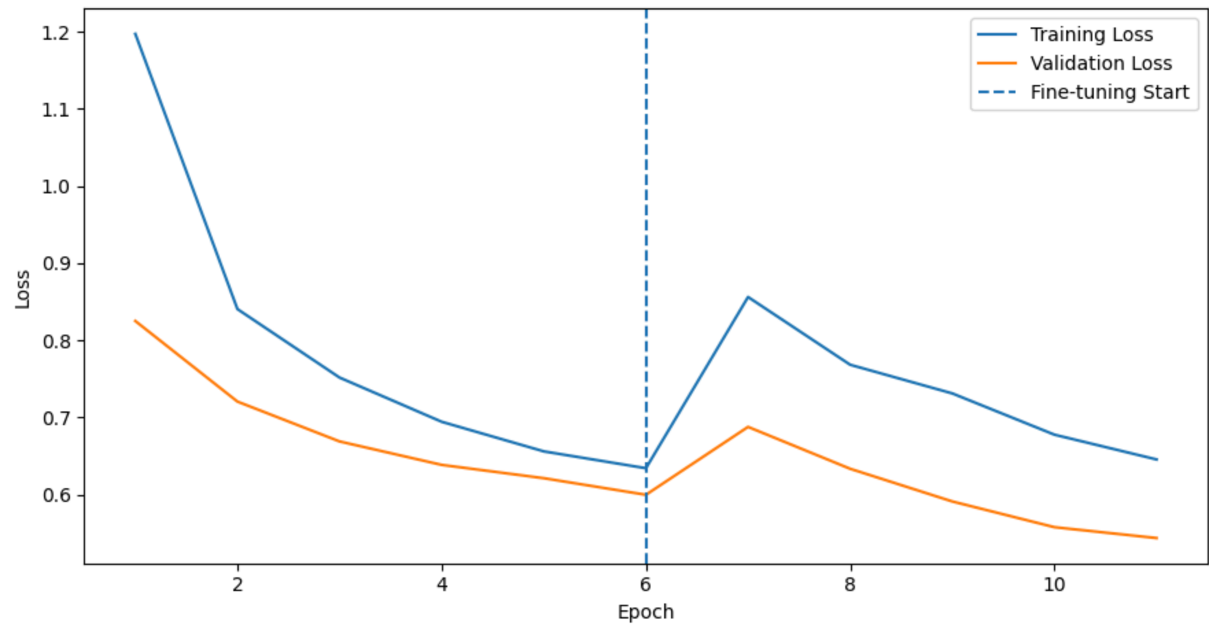
efficientnetv2 Loss
