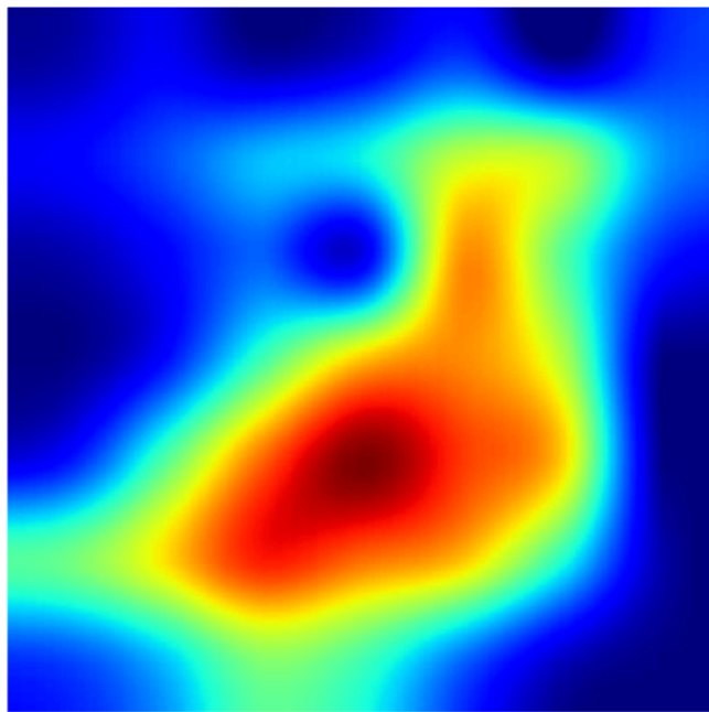
Grad-CAM Heatmap
