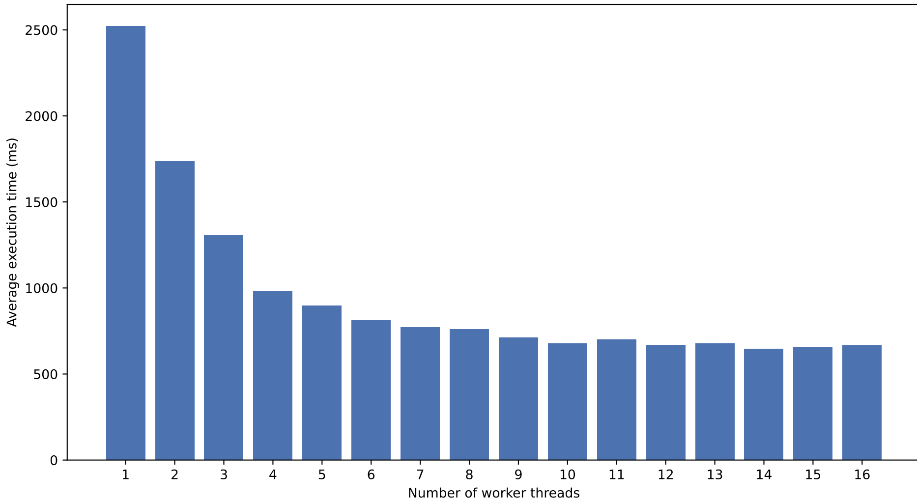
DSGLogBenchmark: INFO-entry analysis of 100 log files (20M INFO / 10M WARN / 10M ERROR entries, 5 repetitions per thread count)
