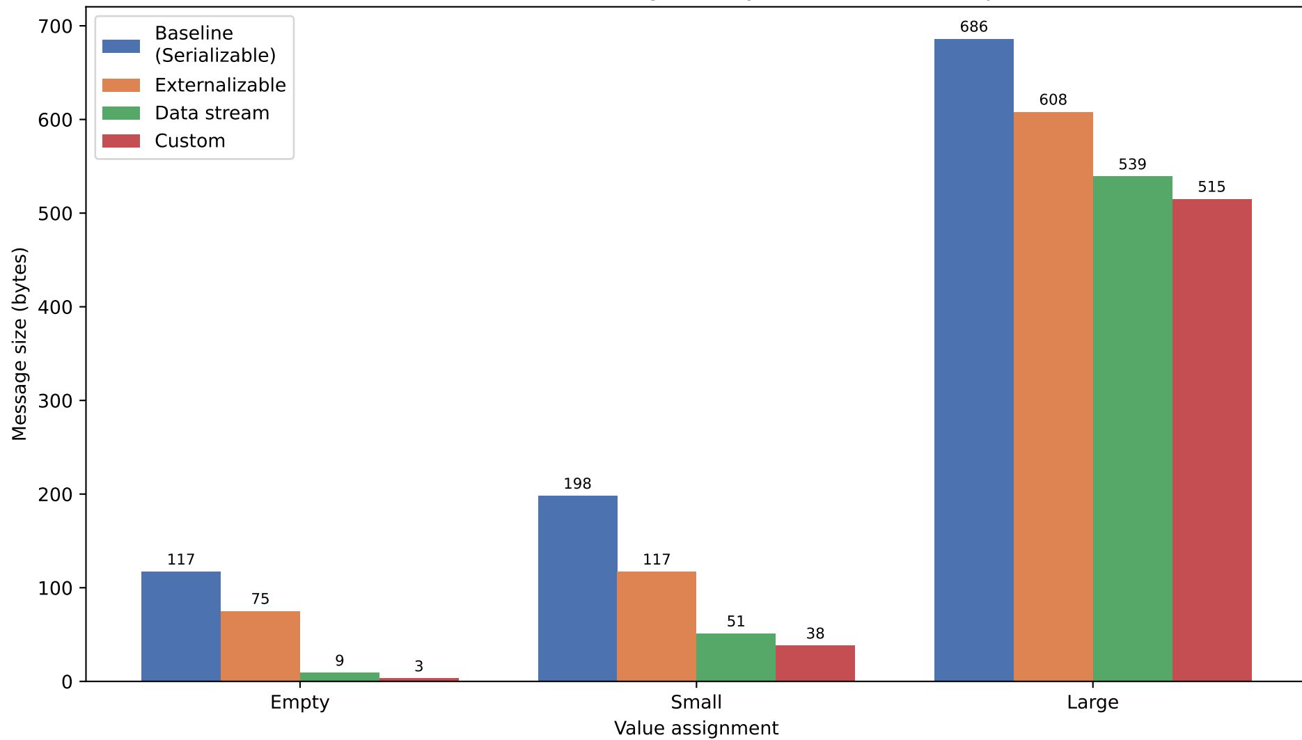
DSGSerialization: message size by serialization technique
