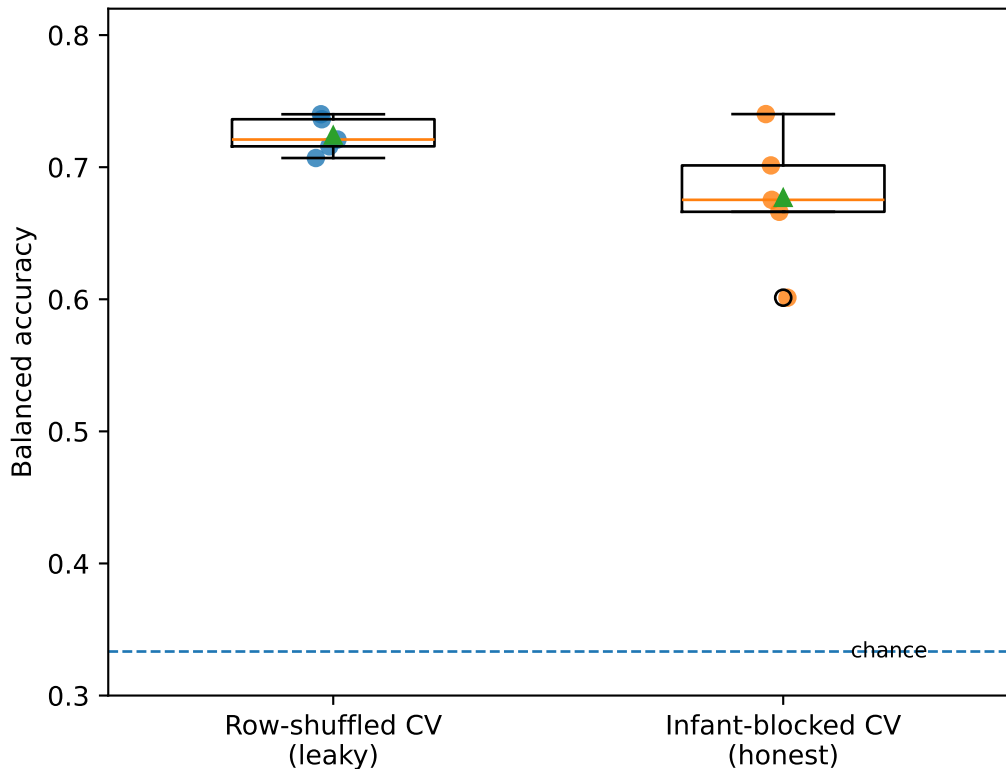
Prediction performance depends on validation design
