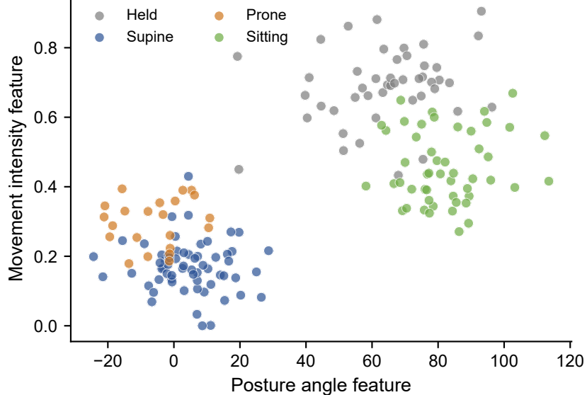
A. Sensor windows occupy separable feature regions
