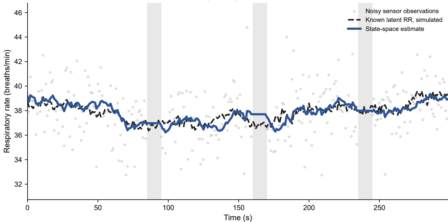
State-space tracking through sensor noise and dropout
