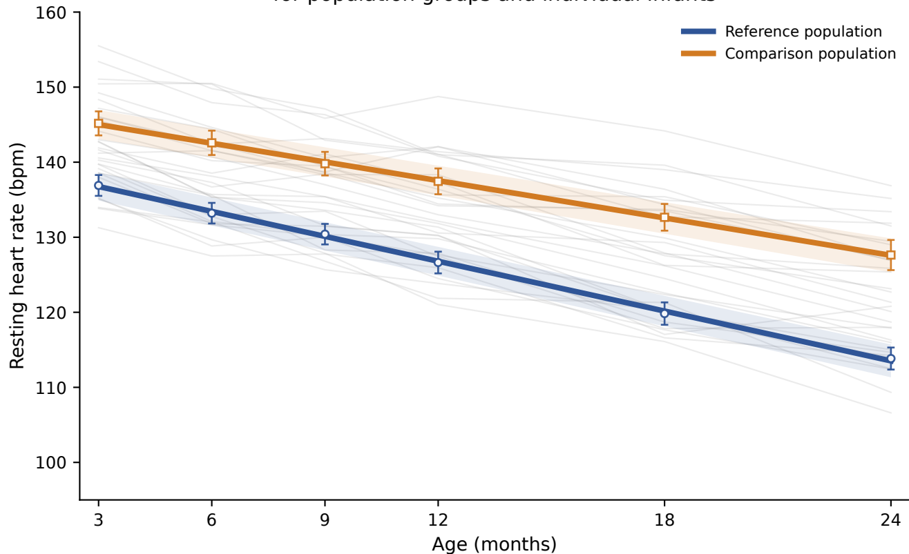
Mixed effects model tracks resting heart rate development for population groups and individual infants
