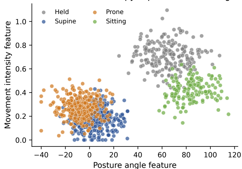
A. Sensor windows occupy separable feature regions
