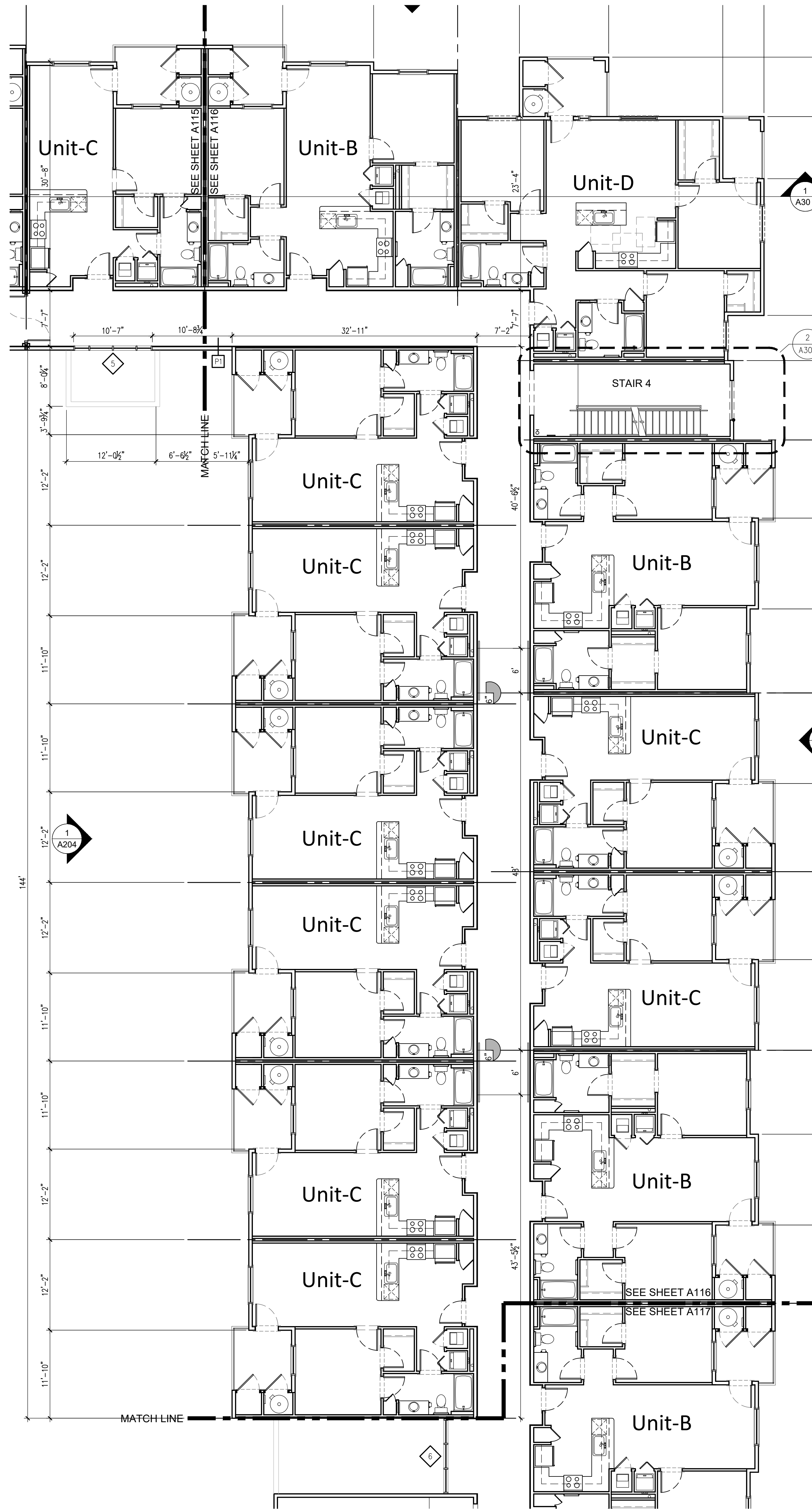
1 PARTIAL 2ND & 3RD FLOOR PLANS SCALE: 1/8" = 1'-0"
