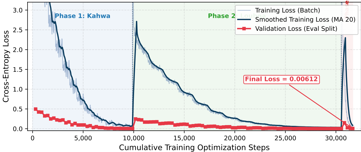
Whisper Medium Cross-Entropy Loss Trajectory across Curriculum
