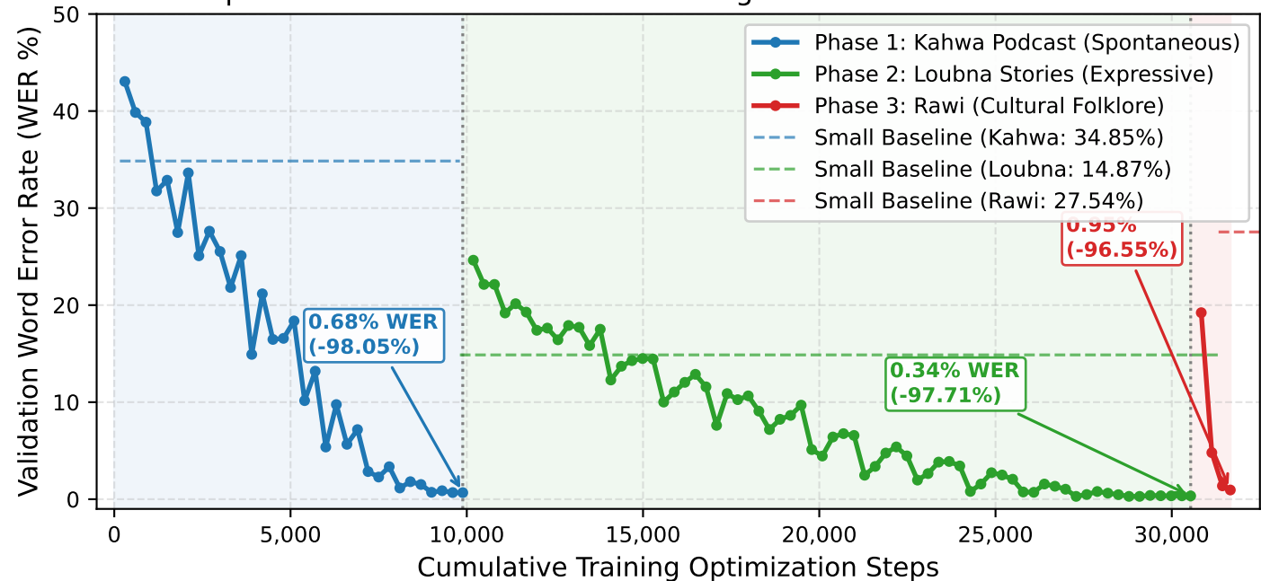
Whisper Medium Validation WER Convergence across Curriculum Phases
