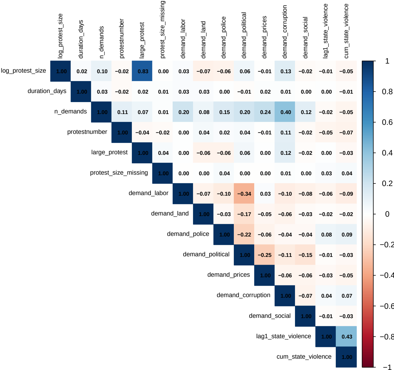
Correlation matrix of candidate regressors
