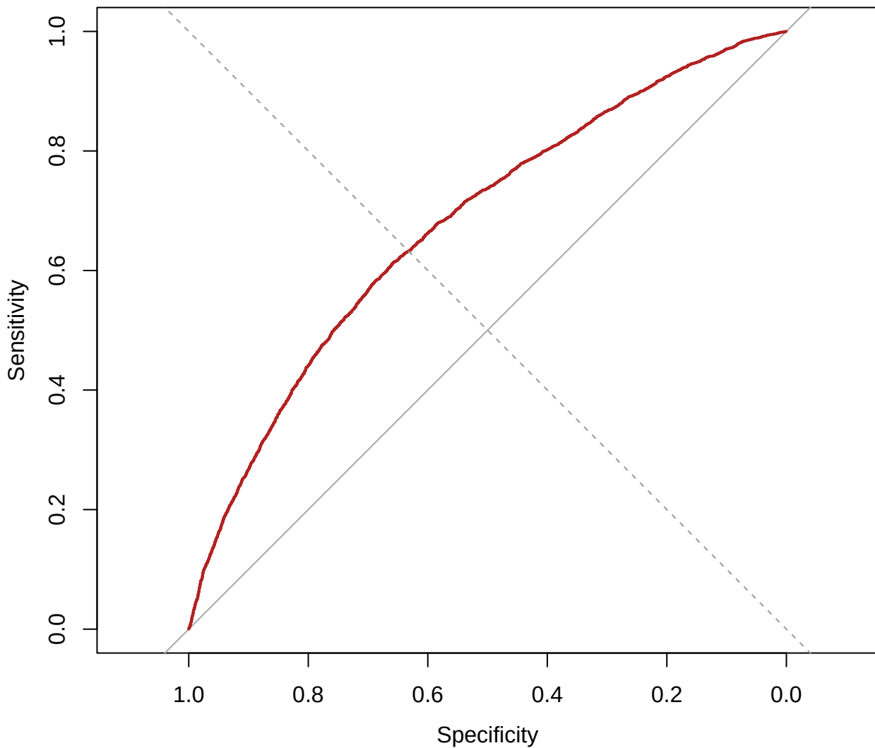
ROC curve – Final logit model (AUC = 0.677 )
