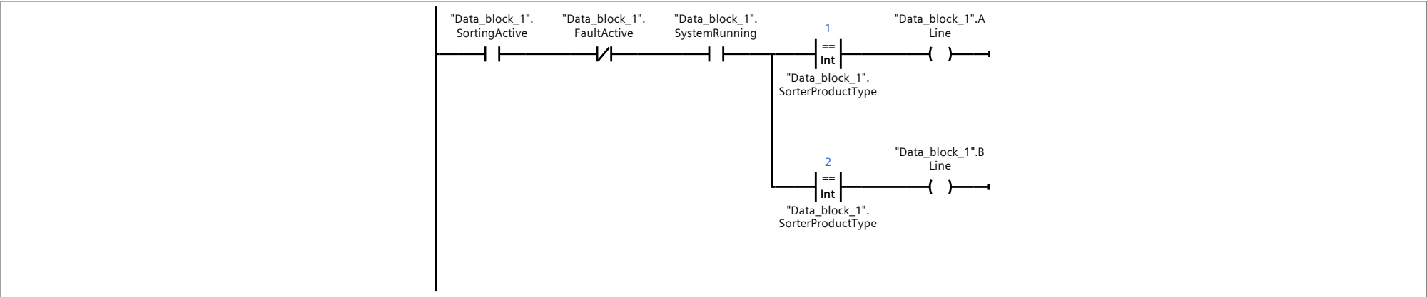
Network 14: Sorting Process and Counters
