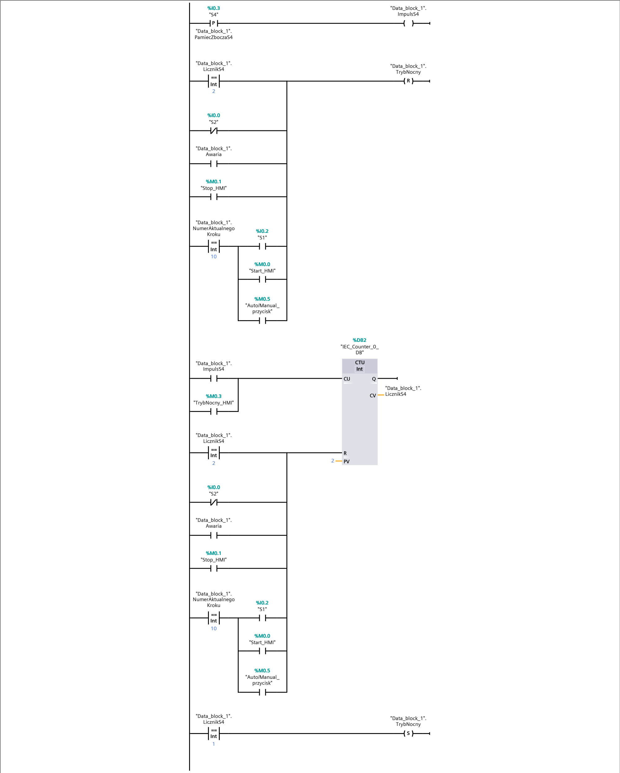
Network 6: Impulsy HMI
