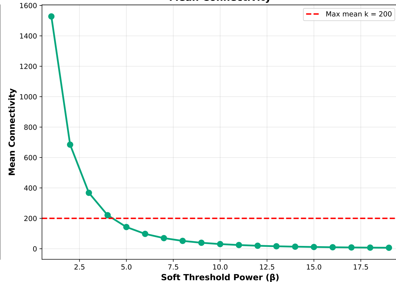
Network Density
