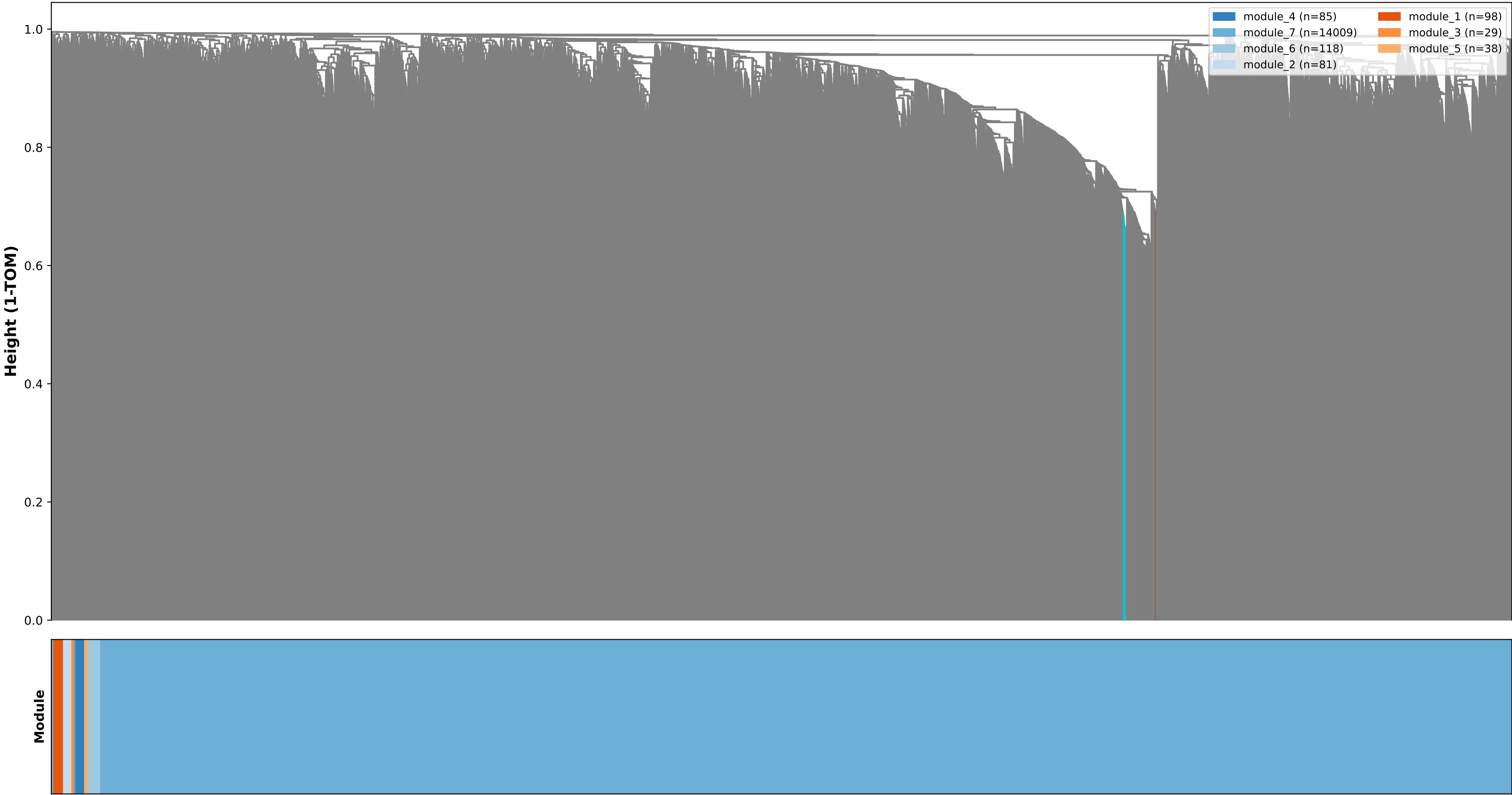
Gene Dendrogram and Module Colors
