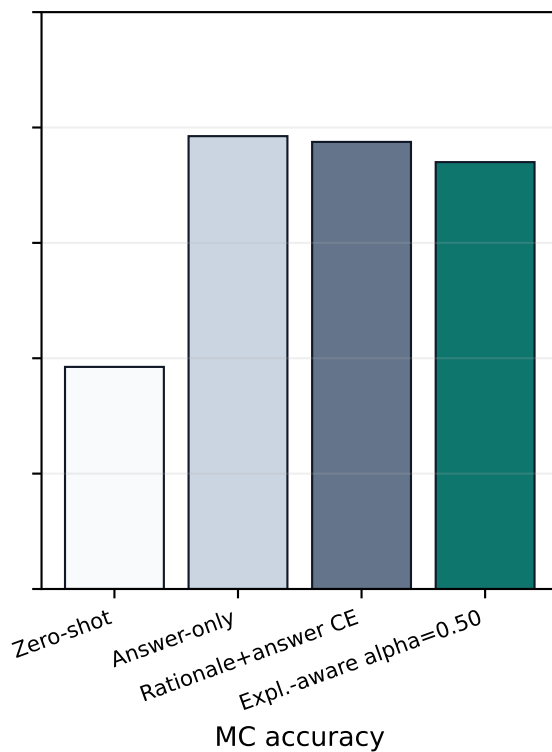
Qwen2-VL / ScienceQA
