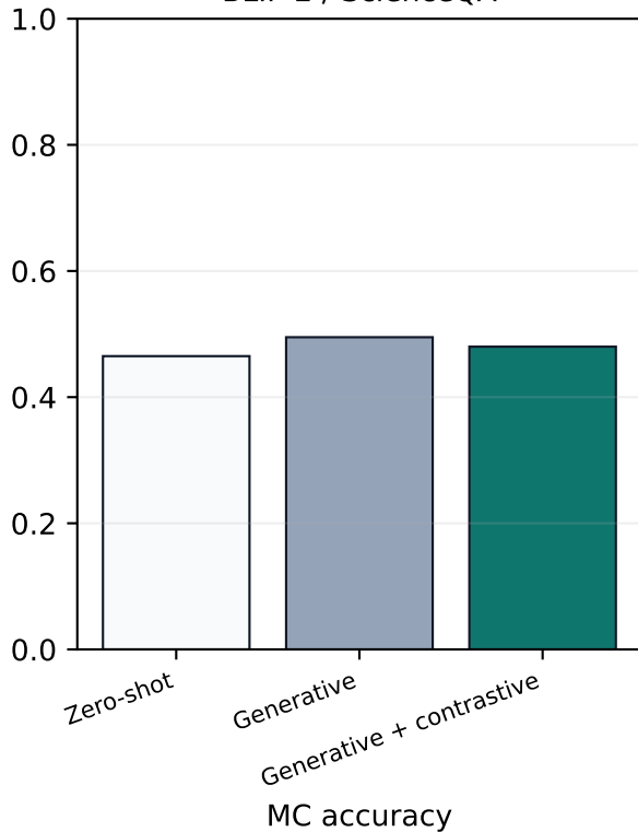
BLIP-2 / ScienceQA
