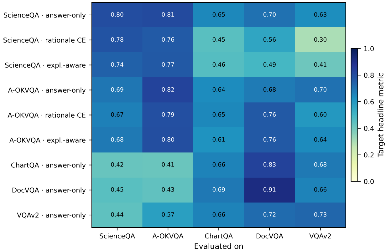
Cross-domain transfer
